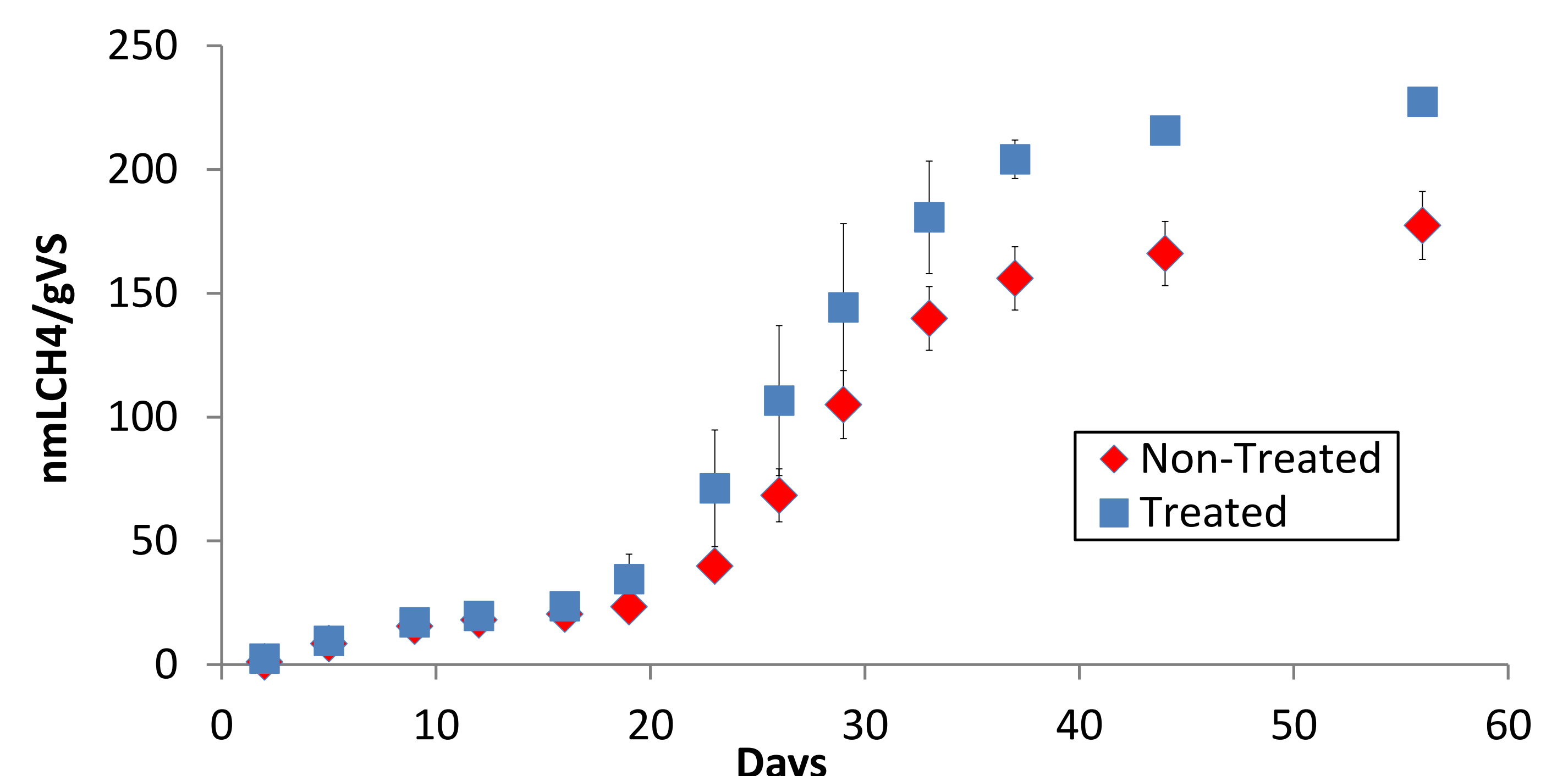
Figure 3. Example of BMP evaluation of pretreatments.
